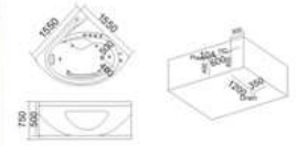
KB-360 1550x1550x750mm
