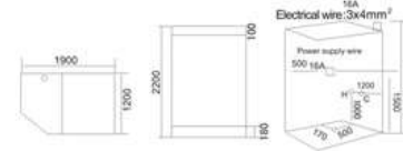
KB-931 1600x1200x2200mm 1700x1200x2200mm 1850x1300x2200mm 1900x1200x2200mm 左右 Left/Right
