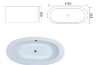
KB-523 1750x850x600mm
