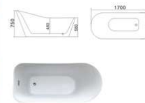
KB-529 1700x800x750mm
