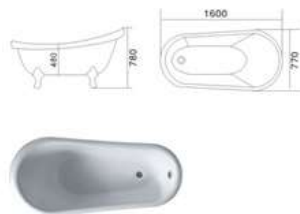
KB-554 1600x770x780mm 1700x800x780mm
