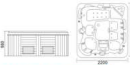
KB-208 2350x2200x980mm
