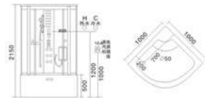
KB-702 1000x1000x2150mm 1100x1100x2150mm
