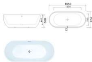
KB-530 1650x700x560mm
