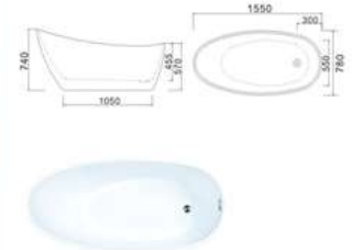
KB-534 1550x780x740mm
