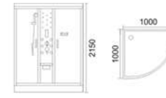
KB-706 900x900x2150mm 1000x1000x2150mm
