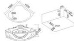
KB-358 1500x1500x700mm
