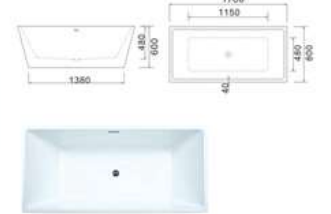
KB-522 1700x800x600mm
