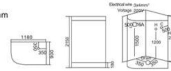
KB-704 1200x900x2150mm
