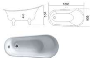
KB-553 1800x900x800mm
