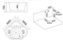
KB-636 1650x1650x750mm
