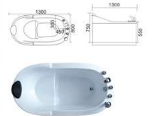
KB-505 1200x800x750mm 1300x800x750mm 1400x800x750mm 1500x800x750mm
