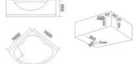
KB-383 1600x1600x650mm
