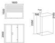
KB-1033 铁杉木 1800x1500x2000mm 可非标订做
